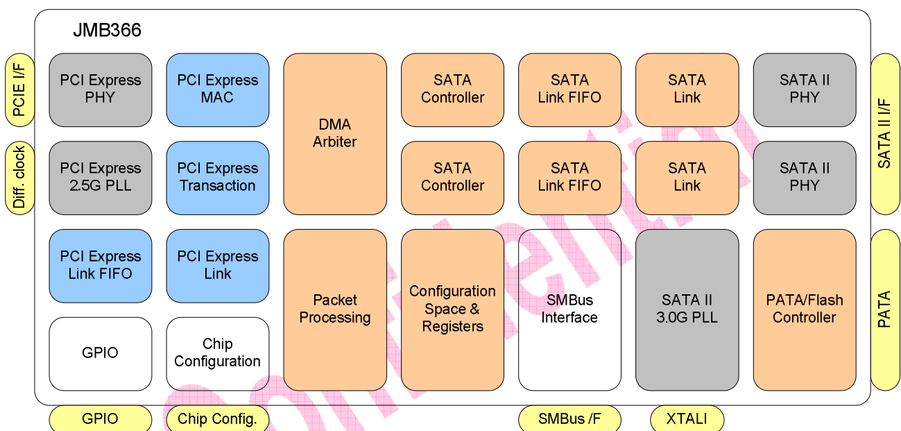
Functional Block Diagram of JMB366
